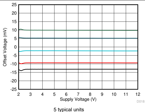
Figure 6-4. Offset Voltage vs Power Supply
