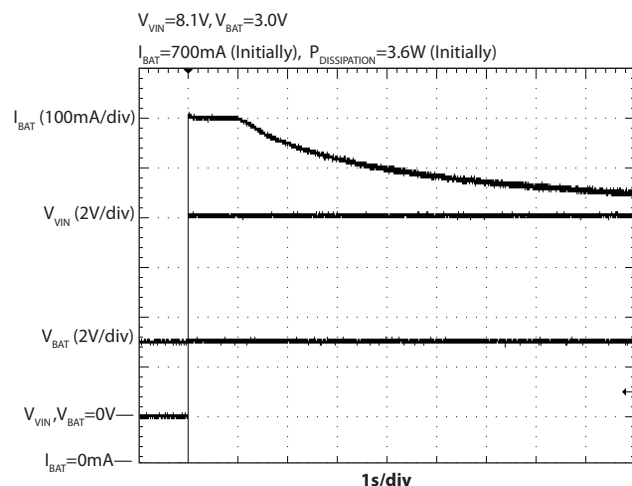
Figure 4 — SC811 Thermal Limiting Example
