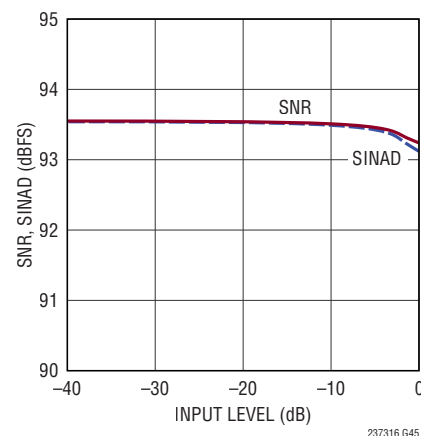
SNR, SINAD vs Input Level, f_{\text{IN}} = 1\text{kHz}
