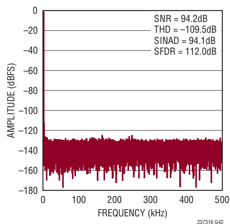
32k Point FFT f_{\text{SAMPL}} = 1\text{MSPS} , f_{\text{IN}} = 1\text{kHz} , REFBUF = 5\text{V}
