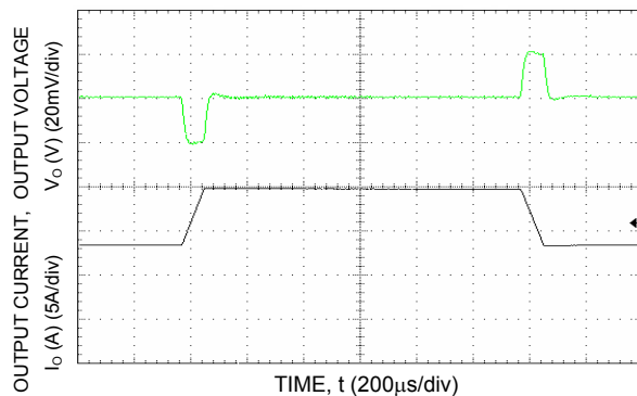
Figure 5. Transient Response to Dynamic Load Change from 50% to 75% to 50% of full load.
