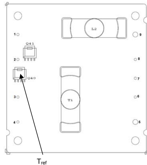
Figure 23. T_{\text{ref}} Temperature Measurement Location.
