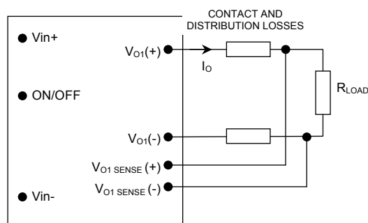
Figure 20. Circuit Configuration for Remote Sense Operation
