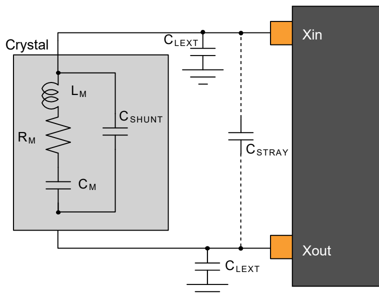
Figure 41-6. Oscillator Connection
