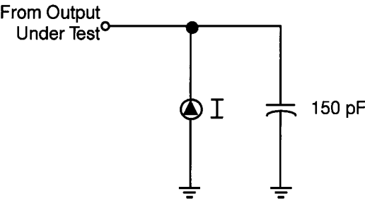
Figure 3. Test Load Diagram
