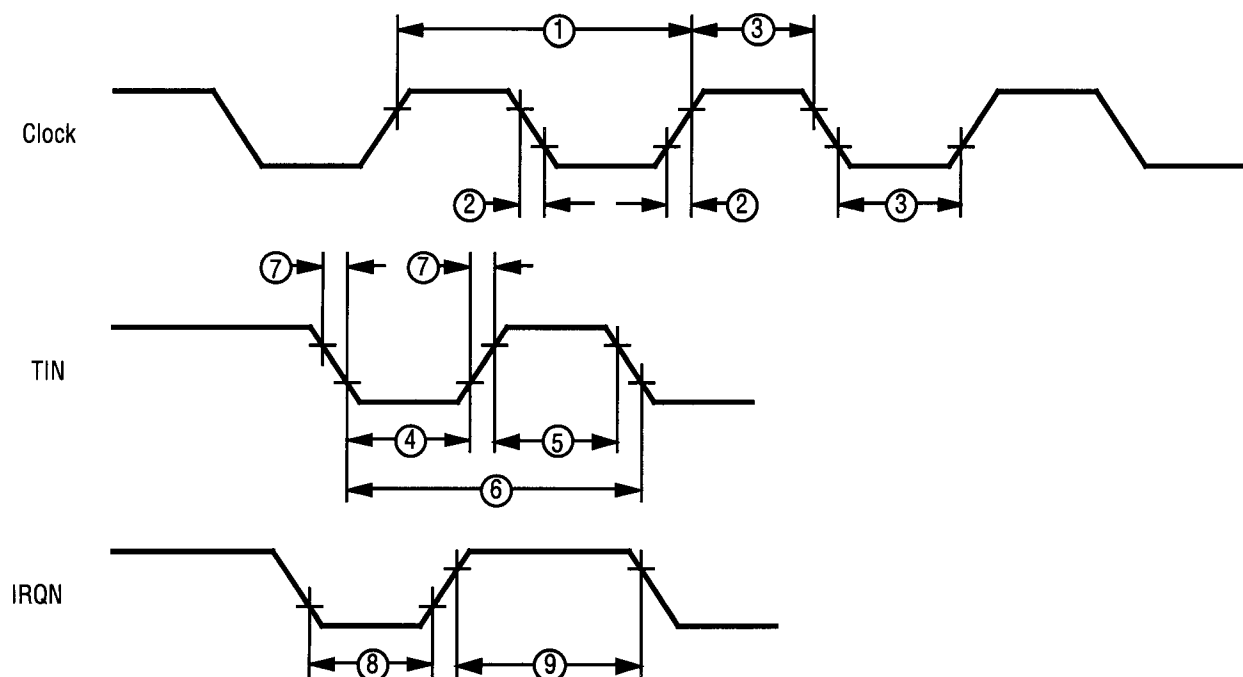
Figure 5. Additional Timing
