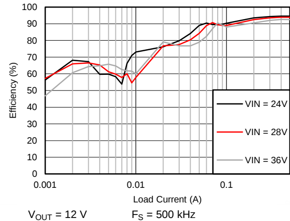
Figure 84. Efficiency
