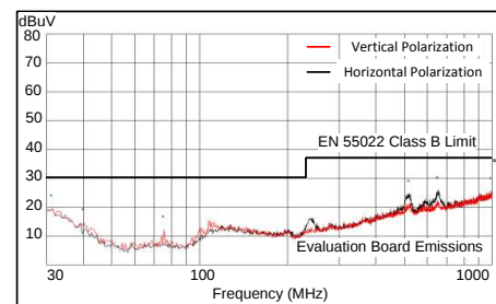
Radiated Emission Graph with V_{IN} = 12 V, V_{OUT} = 3.3 V, F_S = 500 kHz, I_{OUT} = 0.5 A
