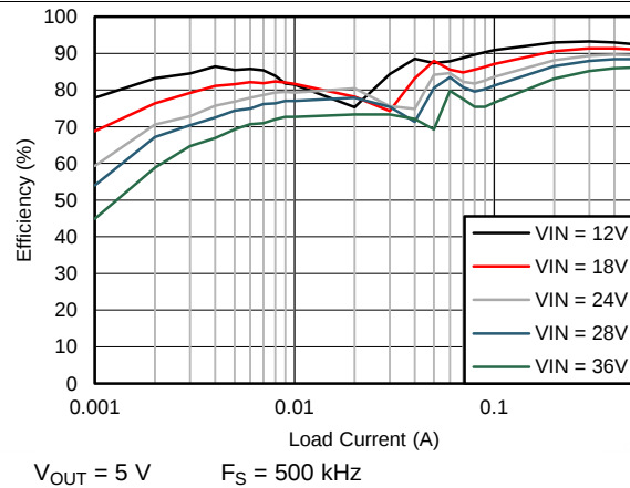
Figure 3. Efficiency
