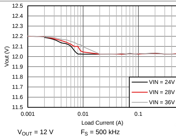
Figure 85. Output Voltage Regulation
