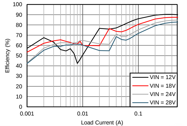
Figure 72. Efficiency
