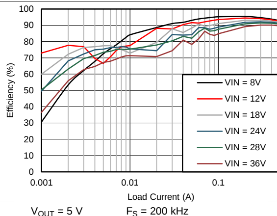
Figure 66. Efficiency
