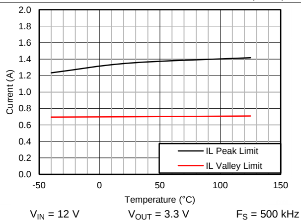
Figure 31. Peak and Valley Current Limits vs Temperature
