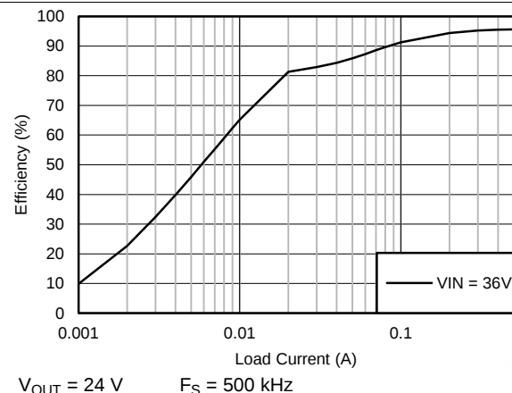
Figure 6. Efficiency
