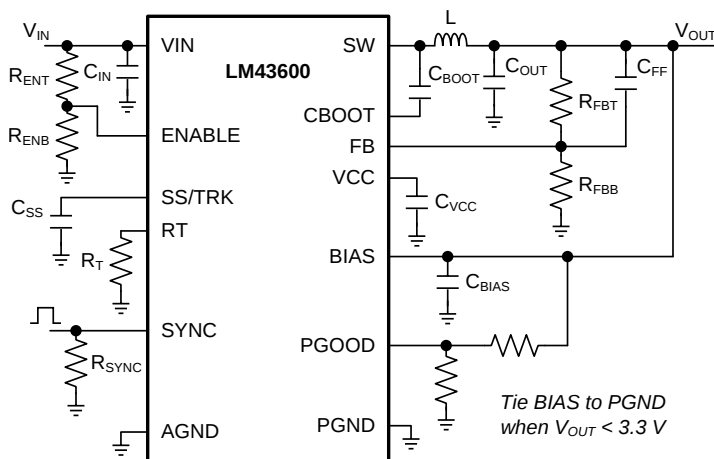
Figure 46. LM43600 Schematic with All Features
