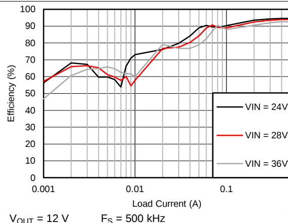
Figure 5. Efficiency
