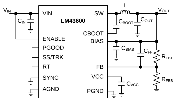
Figure 44. LM43600 Basic Schematic for V_{OUT} \geq 3.3 V, Tie BIAS to V_{OUT}
