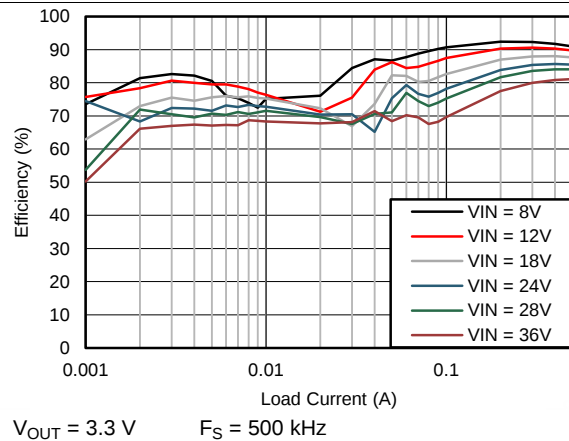
Figure 1. Efficiency
