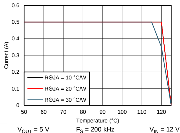
Figure 70. Derating Curve
