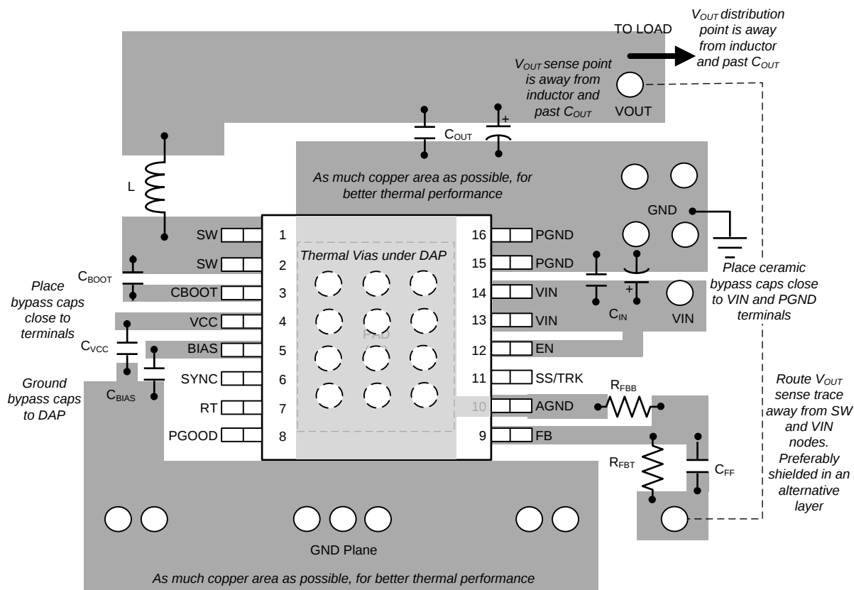
Figure 108. LM43600 PCB Layout Example
