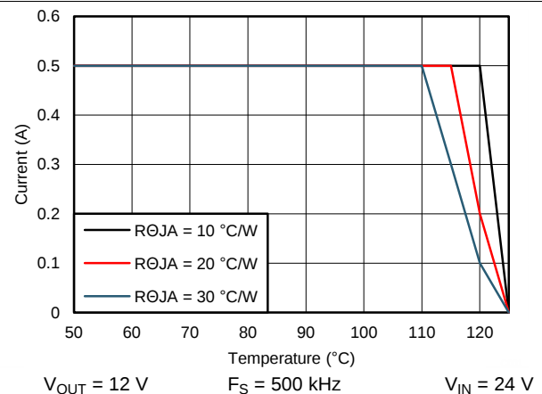
Figure 88. Derating Curve
