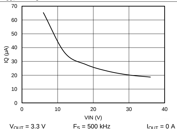
Figure 32. Operation I_Q vs V_{IN} with BIAS Connected to V_{OUT}
