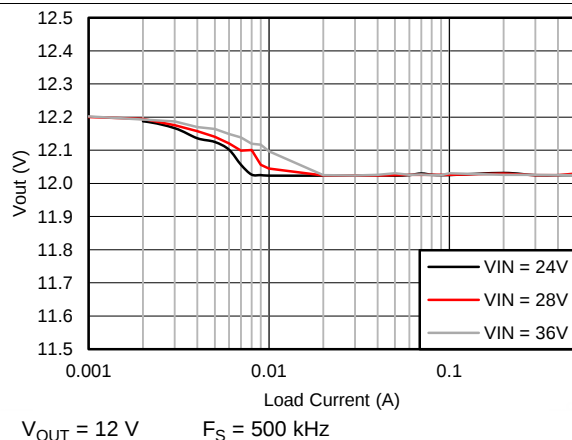
Figure 11. V_{OUT} Regulation
