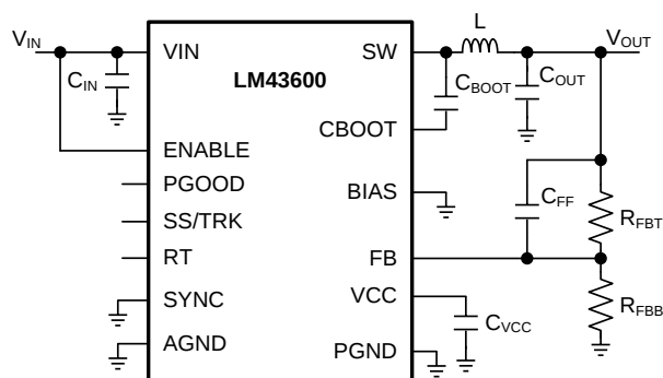
Figure 45. LM43600 Basic Schematic for V_{OUT} < 3.3 V, Tie BIAS to Ground
