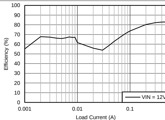
Figure 78. Efficiency
