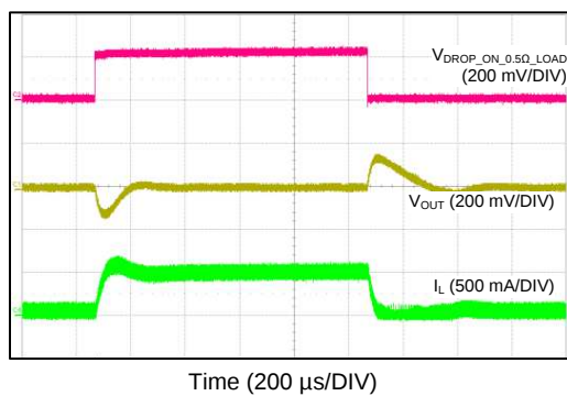
Figure 63. Load Transient Between 0.05 A and 0.5 A
