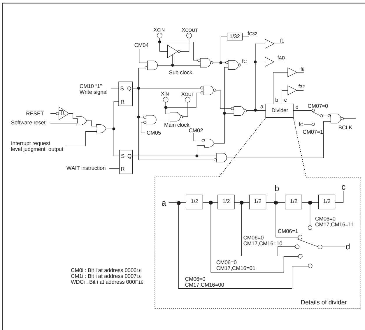
Figure 1.17. Clock generating circuit
