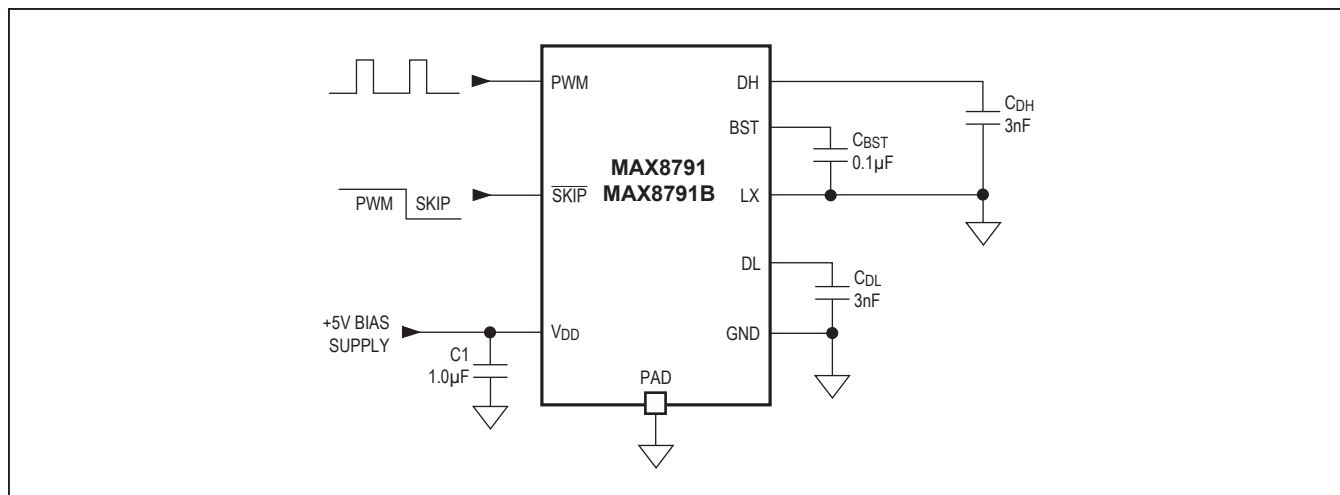
Figure 1. Test Circuit
