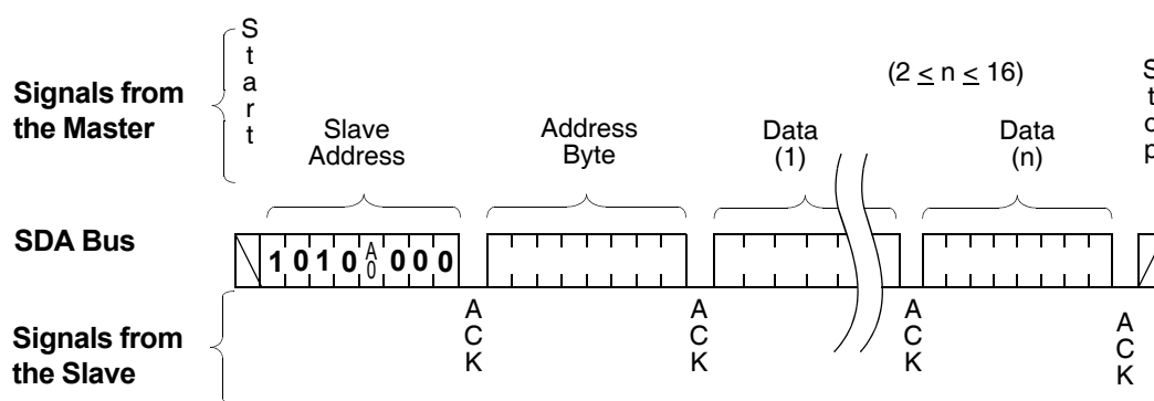
Figure 12. EEPROM Page Write Operation
