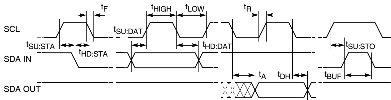
Figure 22. Bus Timing
