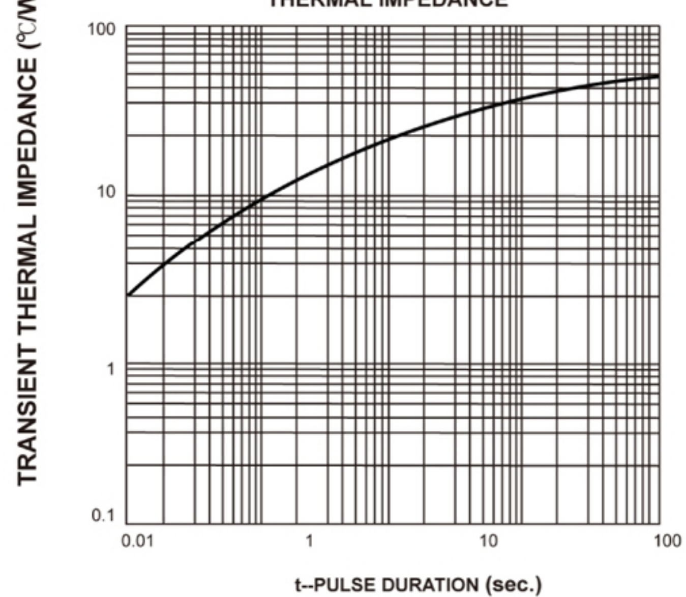
FIG. 6-TYPICAL TRANSIENT THERMAL IMPEDANCE
