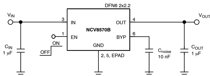
Figure 1. NCV8570B Typical Application Schematic
