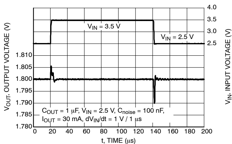
Figure 30. Line Transient Response, V_{OUT} = 1.8 V , C_{OUT} = 1 \mu F , I_{OUT} = 30 mA
