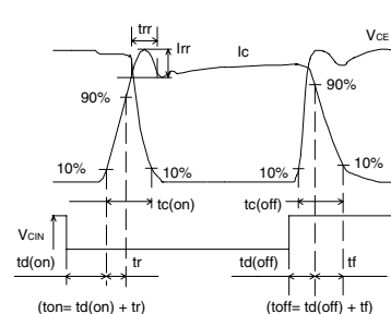
Fig. 4 Switching time test waveform
