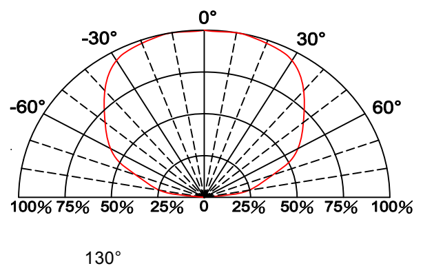
Fig.6 Directive Radiation
