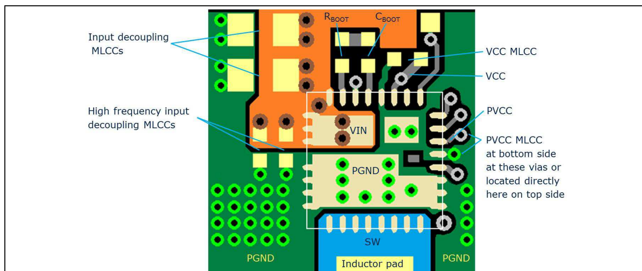
Figure 12 Generic Board Design
