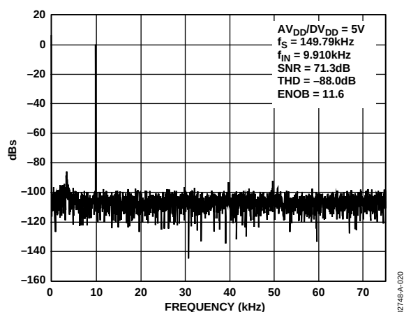
Figure 13. ADuC814 Dynamic Performance at V_{DD} = 5\text{ V}
