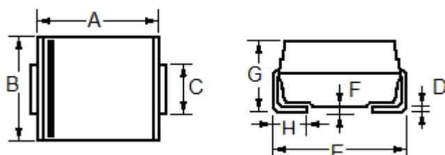
SMC (DO-214AB)
