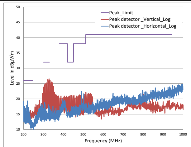
Figure 92. LM73606-Q1 Radiated EMI Result vs. CISPR25 Limits - High Frequency
