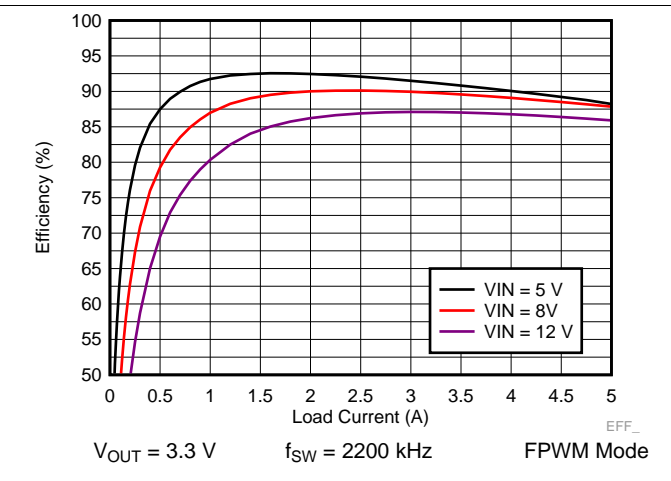
Figure 32. LM73605-Q1 Efficiency
