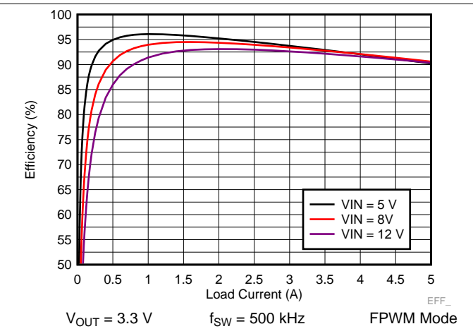
Figure 30. LM73605-Q1 Efficiency
