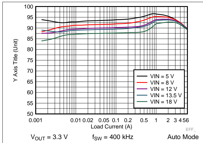
Figure 27. LM73606-Q1 Efficiency
