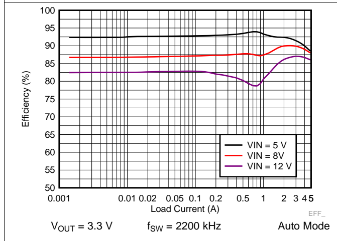
Figure 31. LM73605-Q1 Efficiency
