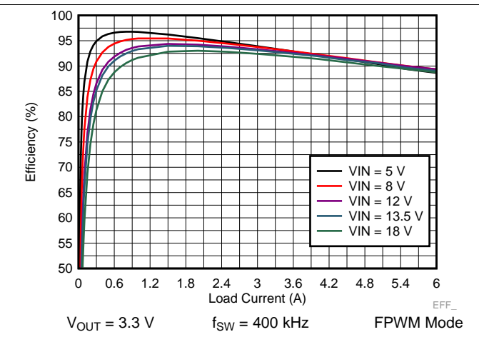
Figure 28. LM73606-Q1 Efficiency
