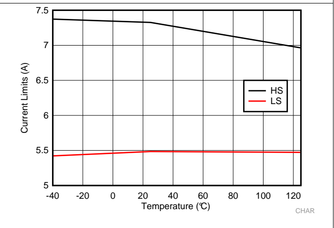
Figure 4. LM73605-Q1 High-Side and Low-Side Current Limits
