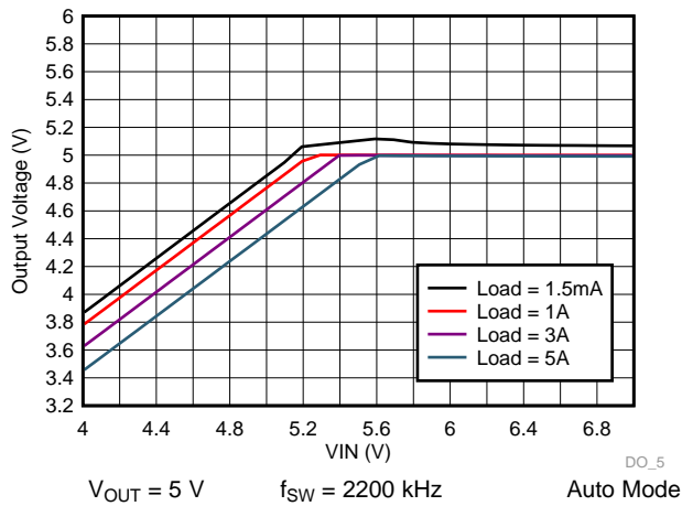
Figure 61. LM73605-Q1 Dropout Curve
