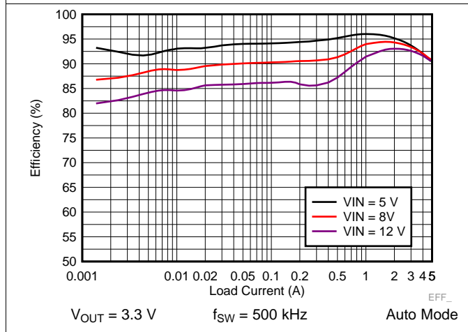
Figure 29. LM73605-Q1 Efficiency
