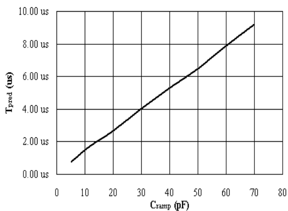
Figure 6 : T pred vs C cramp @ Freq = 20 KHz
