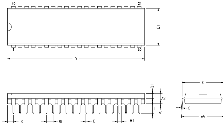
Figure 35. 40-Pin PDIP
