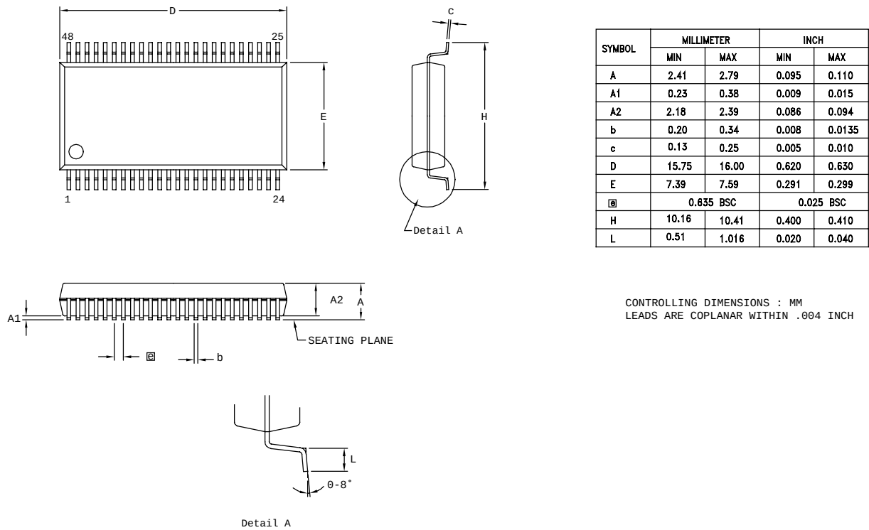
Figure 34. 48-Pin SSOP
