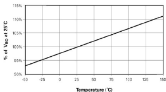
Figure SB4 - Breakover Voltage vs. Temperature
