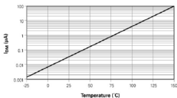
Figure SB6 - Off-state Current vs. Temperature
