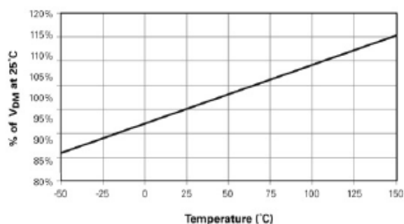
Figure SB3 - Off-state Voltage vs. Temperature
