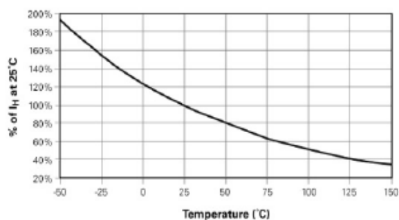
Figure SB5 - Hold Current vs. Temperature
