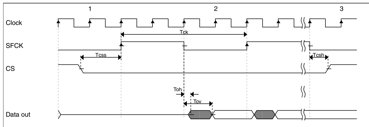
Figure 28. QuadSPI output timing (SDR mode) diagram
