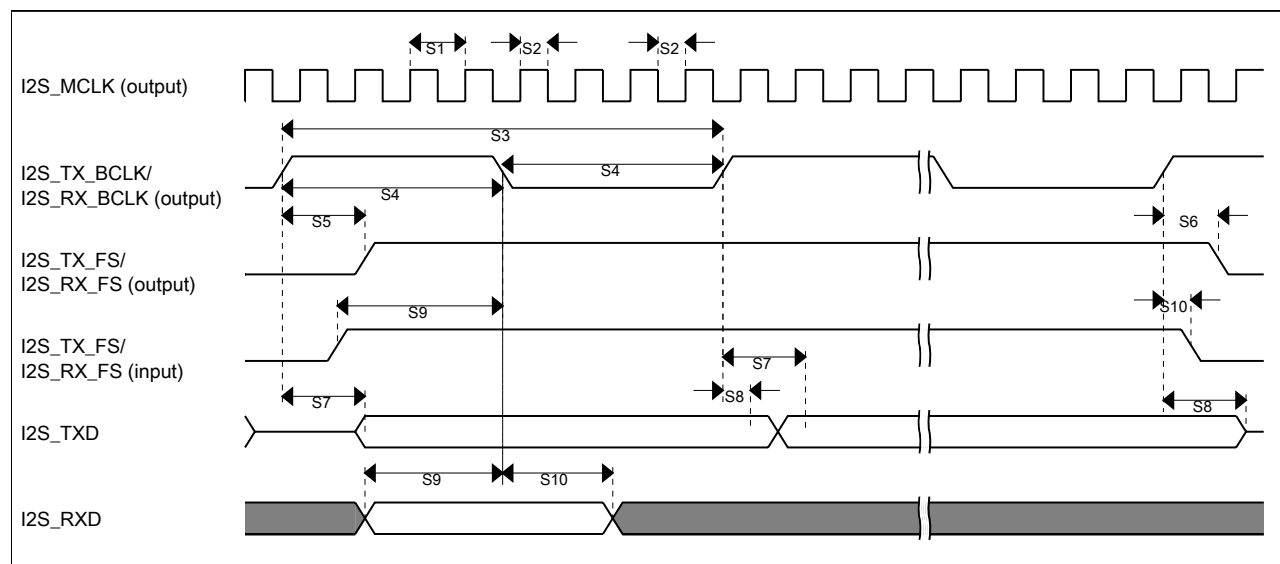
Figure 37. I2S/SAI timing — master modes
