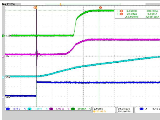
Ch1: Input voltage; Ch2: Soft-start (SS) voltage; Ch3: Input current; Ch4: LED current; Time: 2 ms/div
