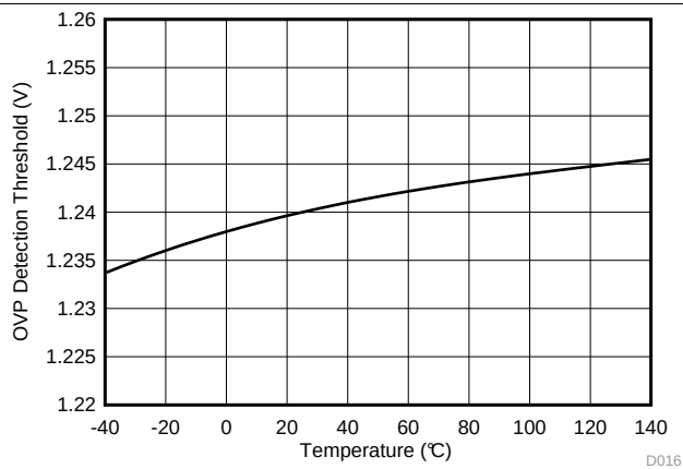
Figure 17. OVP Detection Threshold vs Temperature
