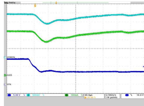
Ch1: Input voltage; Ch2: IMON voltage; Ch3: LED current; Time: 2 ms/div
