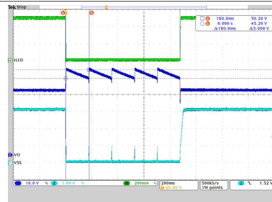
Ch1: Output voltage; Ch2: Soft-start (SS) voltage; Ch4: LED current; Time: 200 ms/div
