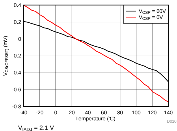
Figure 12. Current Sense Amplifier Offset vs Temperature
