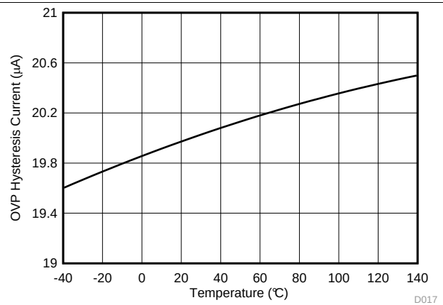
Figure 18. OVP Hysteresis Current vs Temperature
