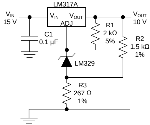
Figure 23. High-Stability 10-V Regulator
