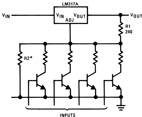
Figure 35. Digitally-Selected Outputs
