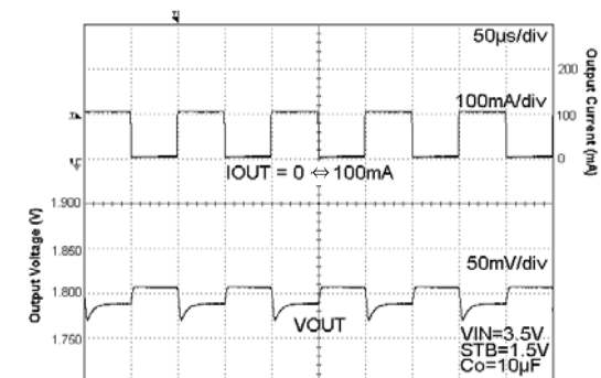
Fig. 57. Load Response Current Pulse=10kHz
