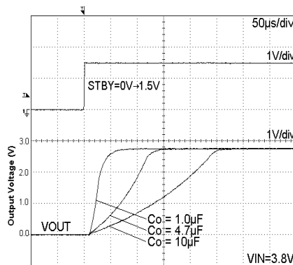
Fig. 32. Start Up Time I_{out} = 200mA
