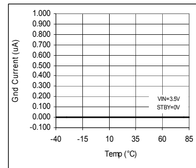
Fig. 48. IGND vs. Temp (STBY)
