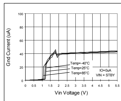
Fig. 39. Circuit Current IGND
