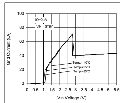
Fig. 13. Circuit Current IGND
