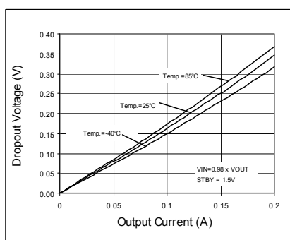
Fig. 14. Dropout Voltage
