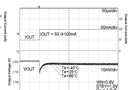
Fig. 25. Load Response
