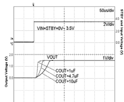
Fig. 91. Startup Time (STBY=VIN) I_{out} = 0 mA
