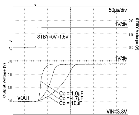
Fig. 31. Start Up Time I_{out} = 0mA
