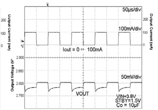
Fig. 28. Load Response Current Pulse=10kHz
