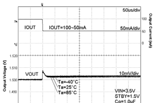
Fig. 84. Load Response
