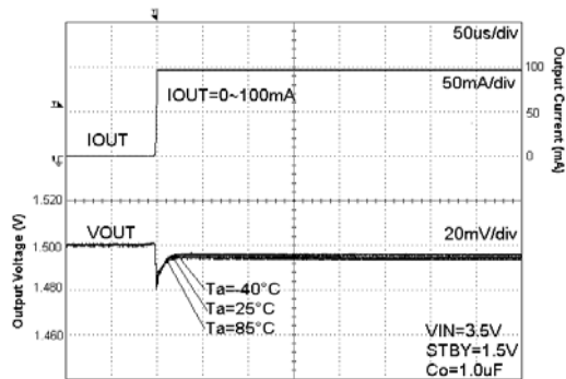
Fig. 81. Load Response
