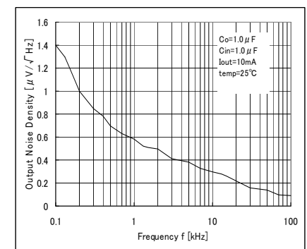
Fig. 22. Output Noise Spectral Density VS. Freq.
