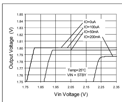
Fig. 38. Line Regulation
