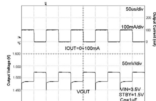
Fig. 85. Load Response Current Pulse=10 kHz
