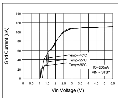
Fig. 40. Circuit Current IGND
