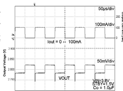
Fig. 27. Load Response Current Pulse=10kHz
