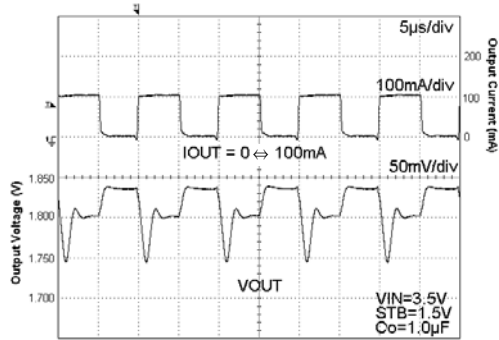
Fig. 58. Load Response Current Pulse=100kHz
