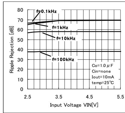
Fig. 79. Ripple Rejection vs. VIN ( I_{out}=10\text{ mA} )
