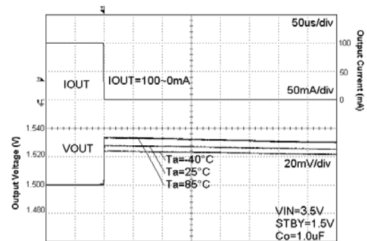
Fig. 82. Load Response
