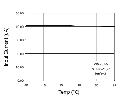
Fig. 76. IGND vs. Temp
