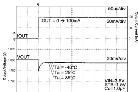
Fig. 52. Load Response
