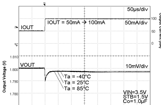
Fig. 54. Load Response
