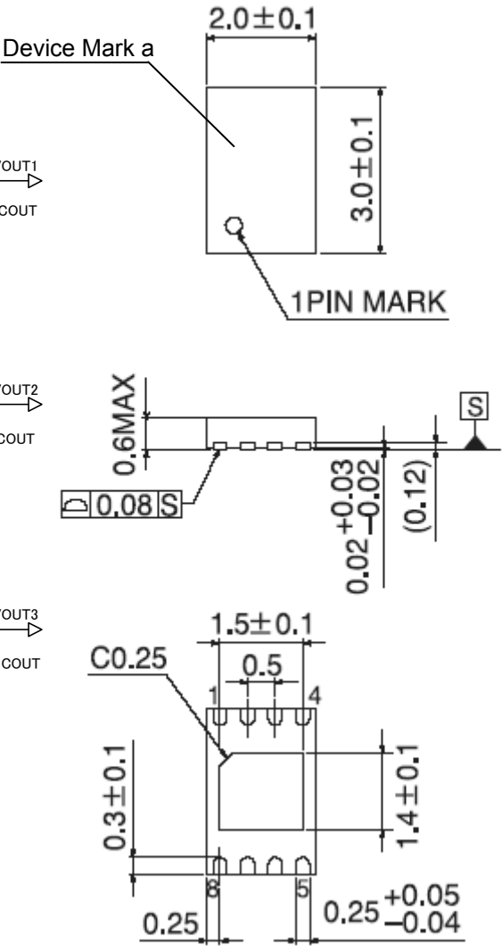
Fig.2 PACKAGE DIMENSIONS
