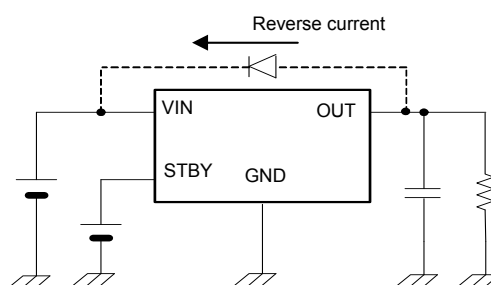
Fig.96 Example of bypass diode connection
