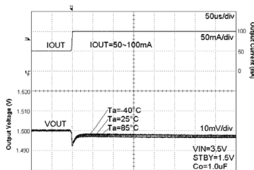
Fig. 83. Load Response
