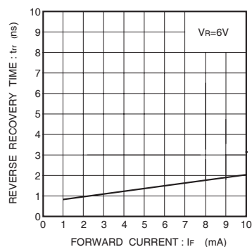
Fig.2 Reverse recovery time
