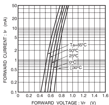
Fig.3 Forward characteristics
