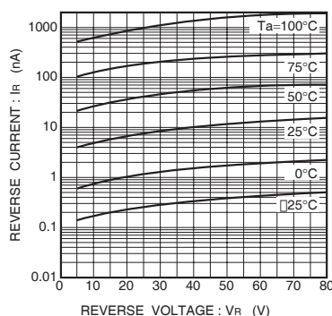
Fig.4 Reverse characteristics
