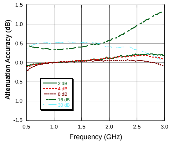
Attenuation Accuracy
