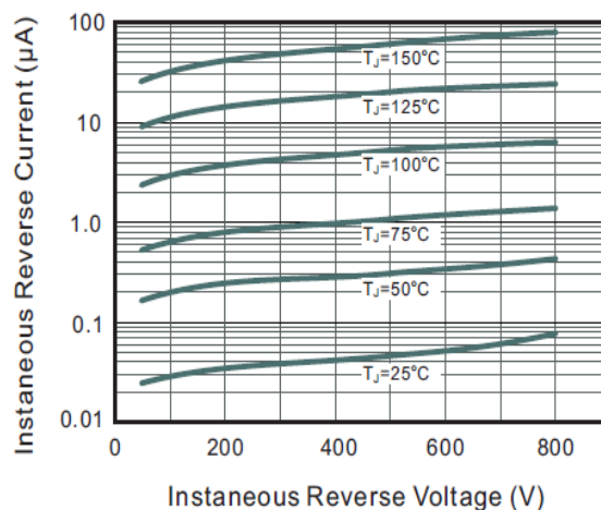
Fig.2 Typical Instantaneous Reverse Characteristics
