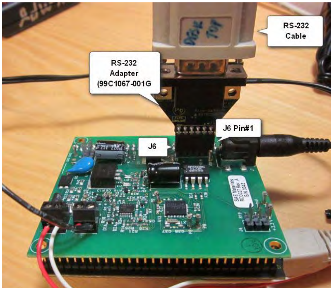
Figure 6. Power Board with Zilog UART-to-Serial Adapter
