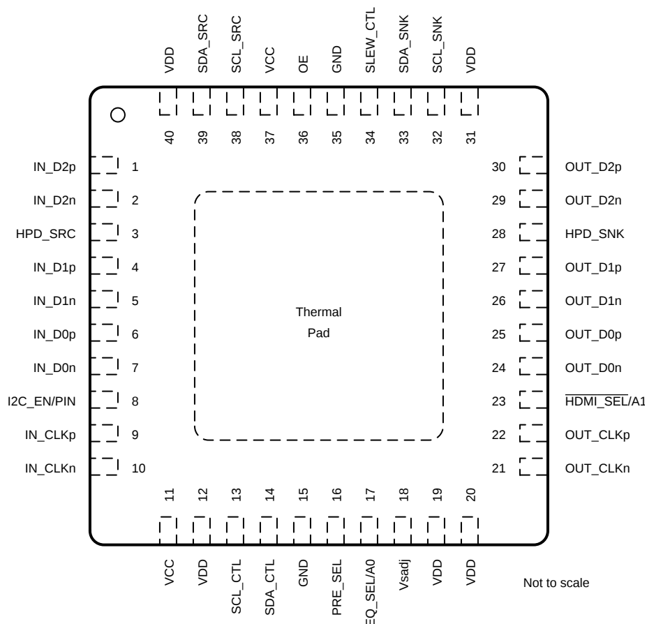
Pin Functions
