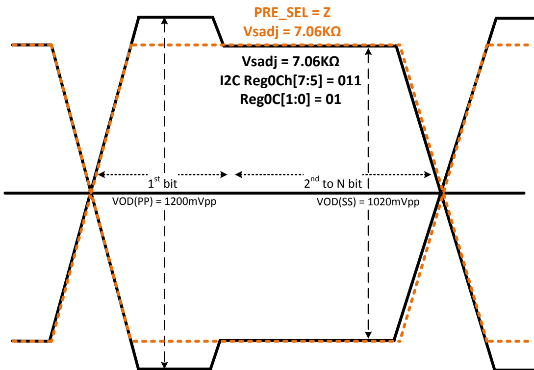
图 29. Pre-Emphasis Using I²C Method
