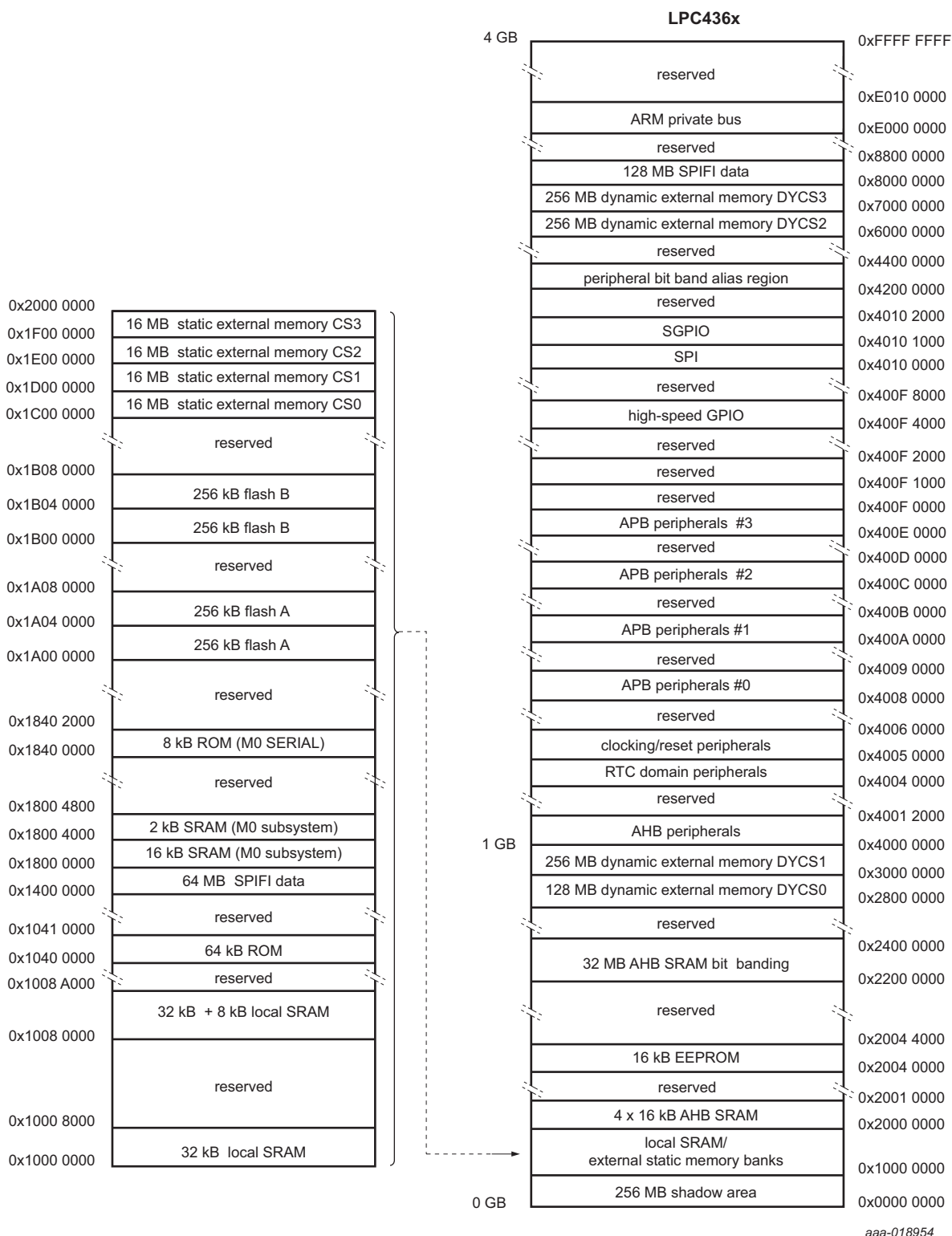
Fig 6. LPC436x Memory mapping (overview)
