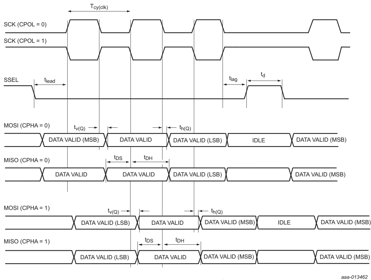
Fig 30. SSP in SPI mode and SPI master timing
