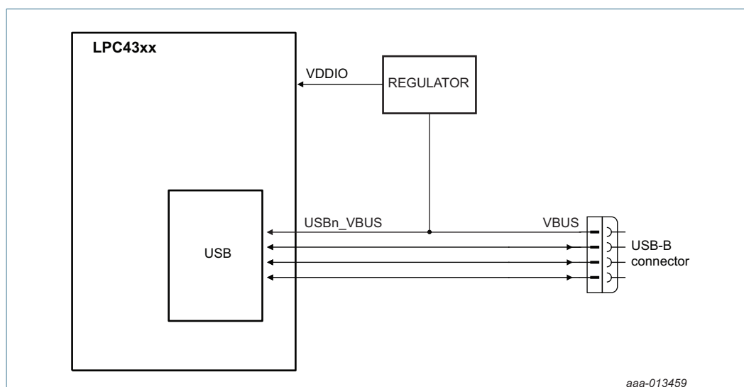
Fig 48. USB interface on a bus-powered device
