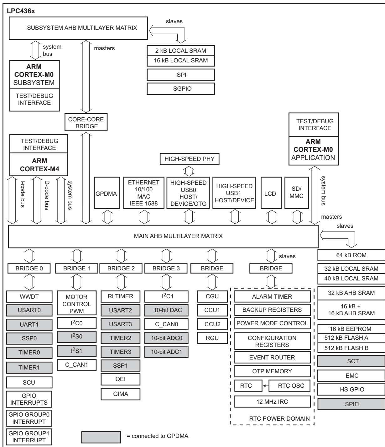
Fig 1. LPC436x Block diagram
