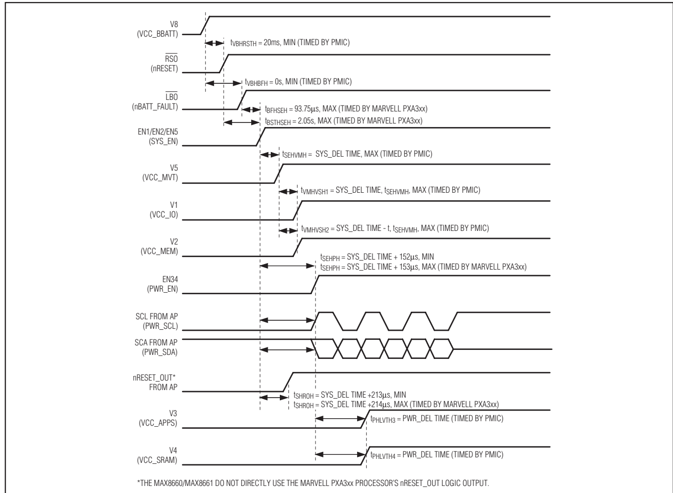
Figure 6. Power-Up Timing
