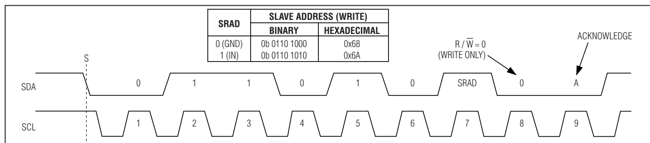
Figure 10. Slave Address Byte
