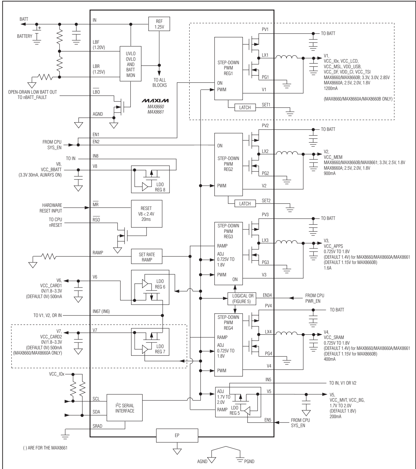
Figure 2. Functional Diagram
