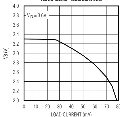
REG8 LOAD REGULATION
