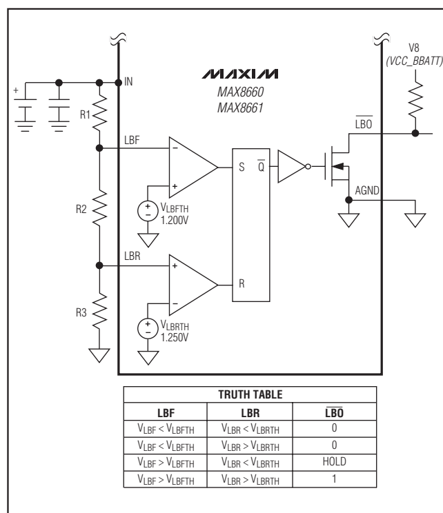
Figure 7. Low-Battery Detector Functional Diagram
