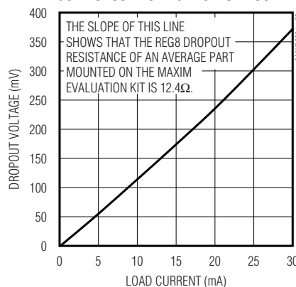
REG8 DROPOUT VOLTAGE vs. LOAD CURRENT
