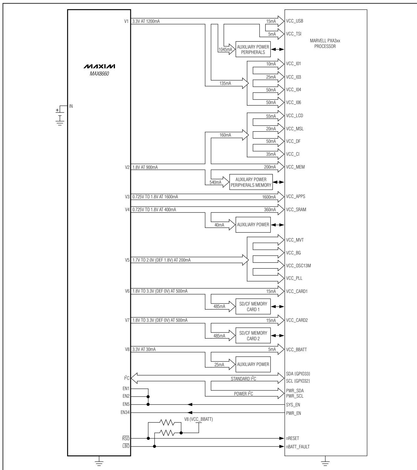
Figure 1. Example MAX8660 Connection to Marvell's PXA3xx Processor. This is one example only. Other connections are also supported.
