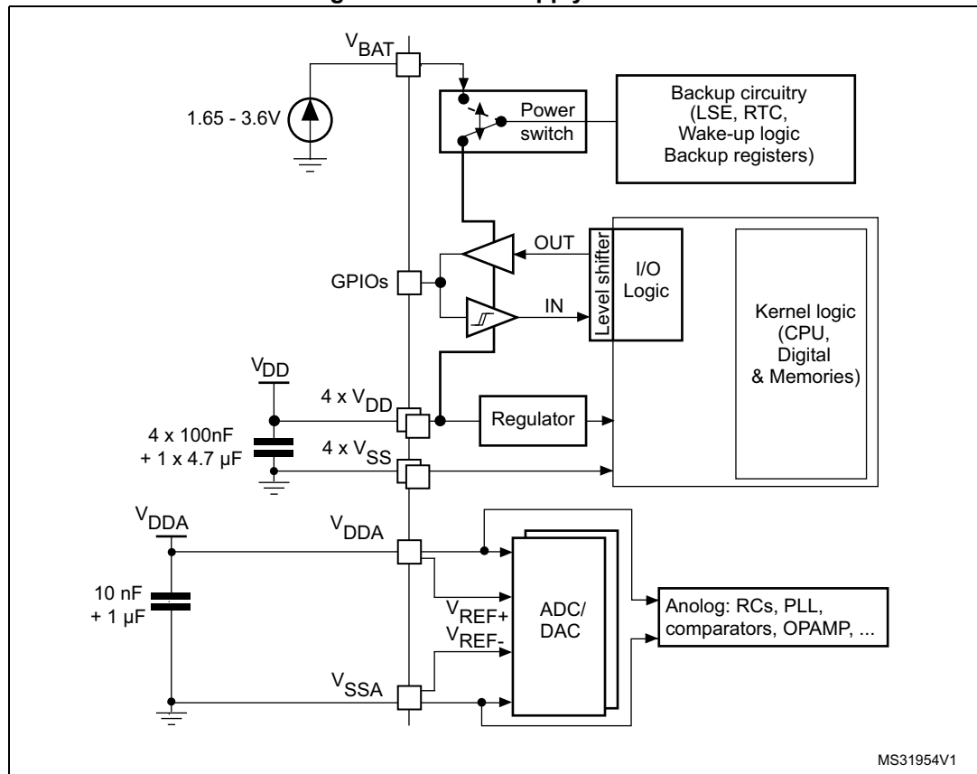
Figure 11. Power-supply scheme
