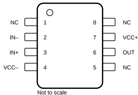
Figure 5-2. TL071H D Package 8-Pin SOIC Top View
