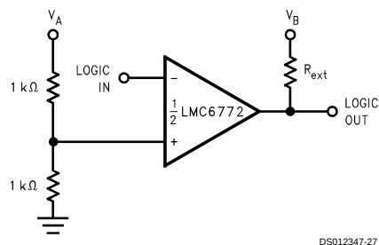
FIGURE 4. Universal Logic Level Shifter
