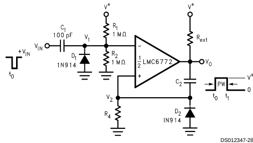
FIGURE 5. One-Shot Multivibrator
