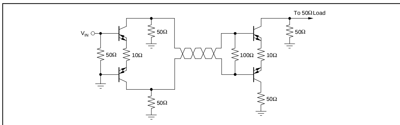
Figure 39. Twisted-Pair Differential Driver and Receiver with the OPA861
