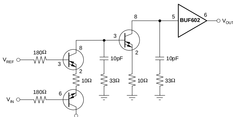
Figure 34. Control-Loop Amplifier Using Three OPA861s
