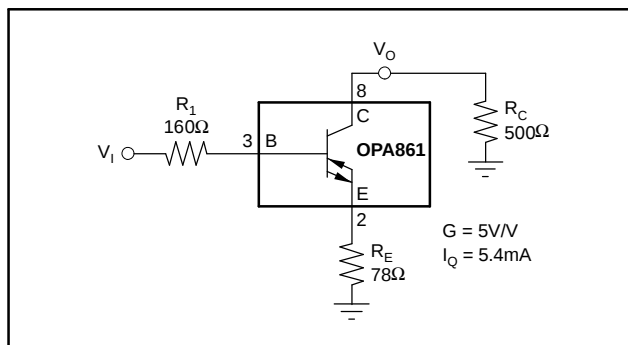
Figure 30. Forward Amplifier Configuration and Test Circuit
