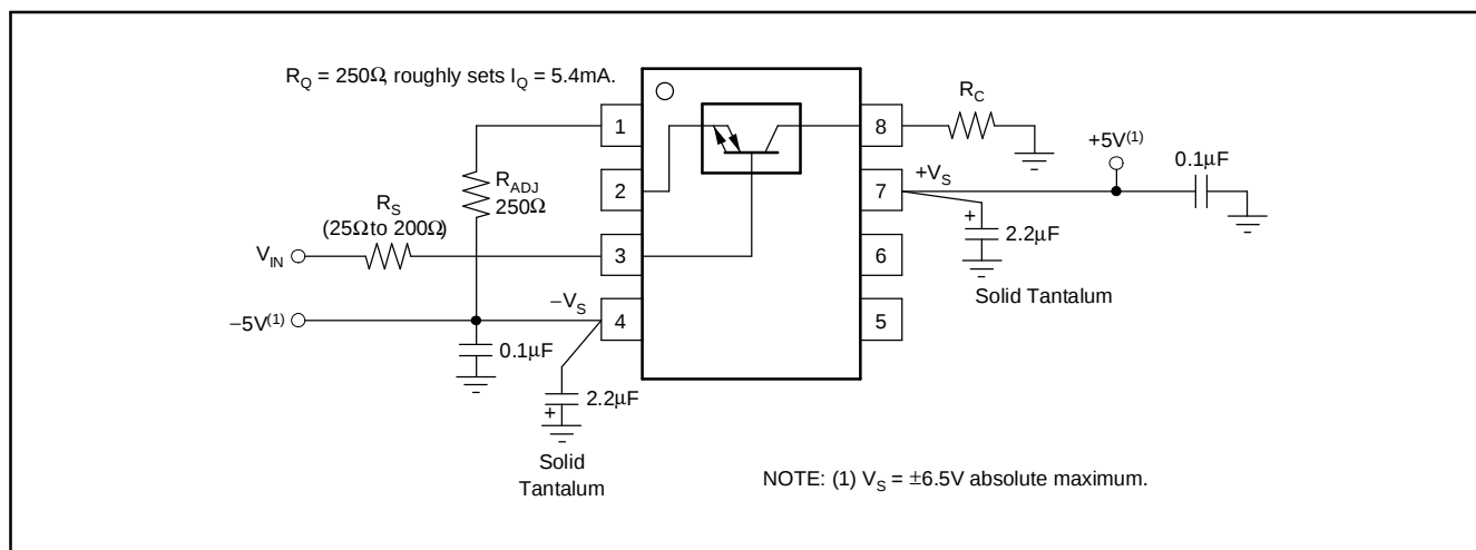
Figure 27. Basic Connections
