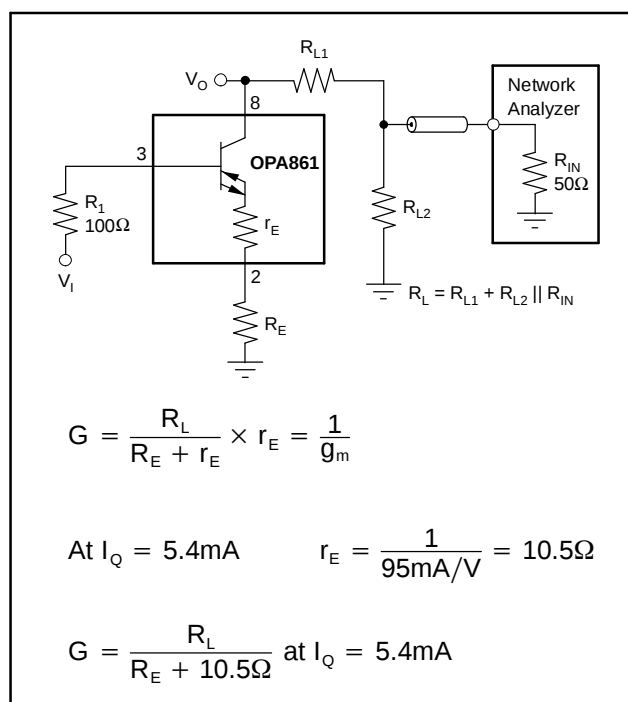
Figure 31. Forward Amplifier Design Equations
