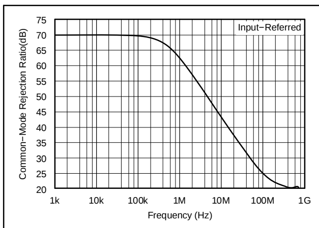
Figure 47. CMRR of the ADC Driver
