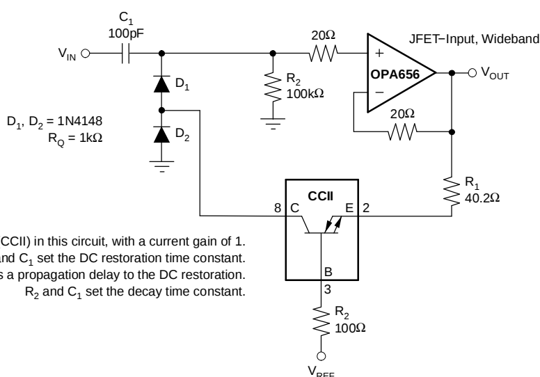
Figure 35. DC Restorer Circuit
