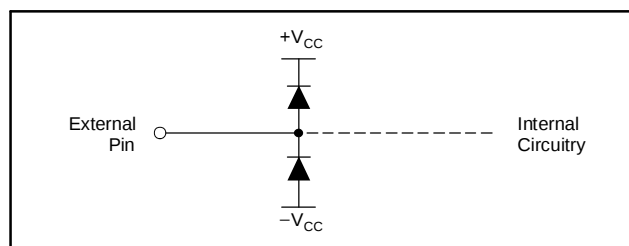
Figure 49. Internal ESD Protection
