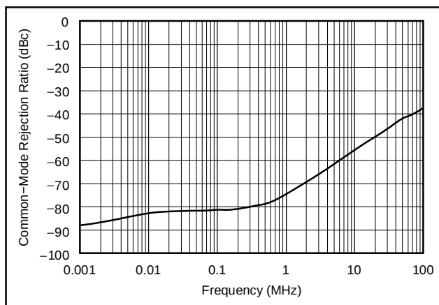
Figure 38. Differential Driver Common-Mode Rejection Ratio for 2V PP Input Signals
