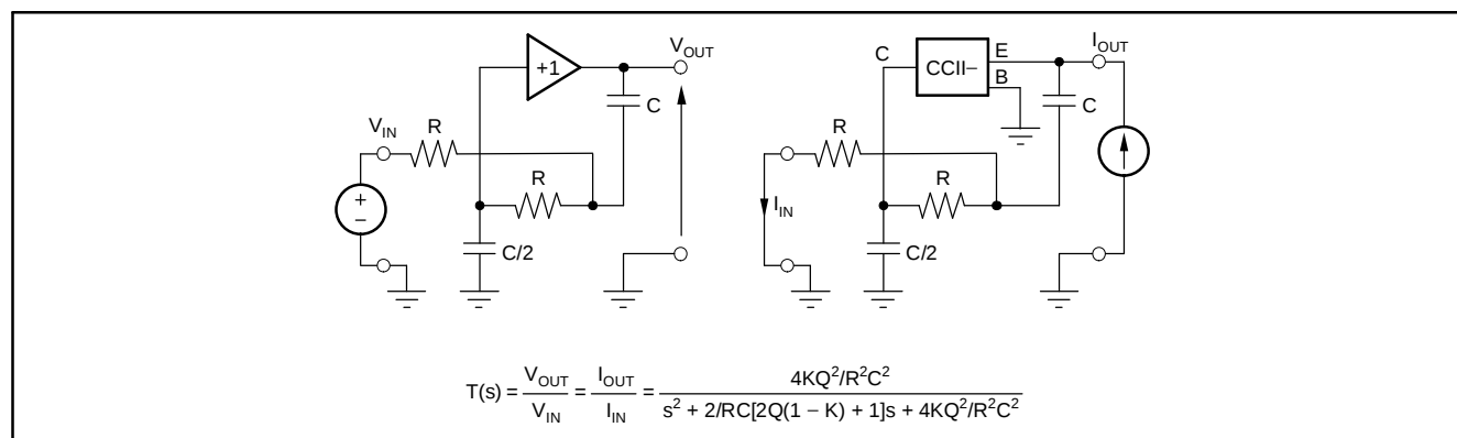
Figure 40. Current Conveyor
