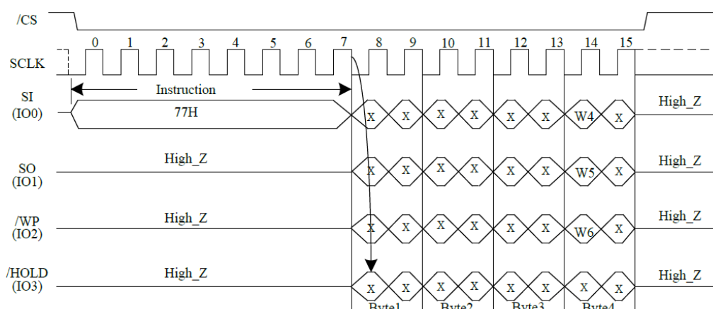
Figure17. Set Burst with Wrap Sequence Diagram
