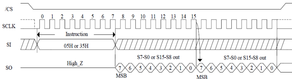
Figure4. Read Status Register Sequence Diagram
