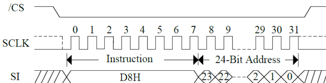
Figure35. 64KB Block Erase Sequence Diagram
