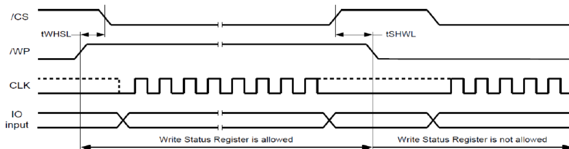
Figure 45. WP Timing
