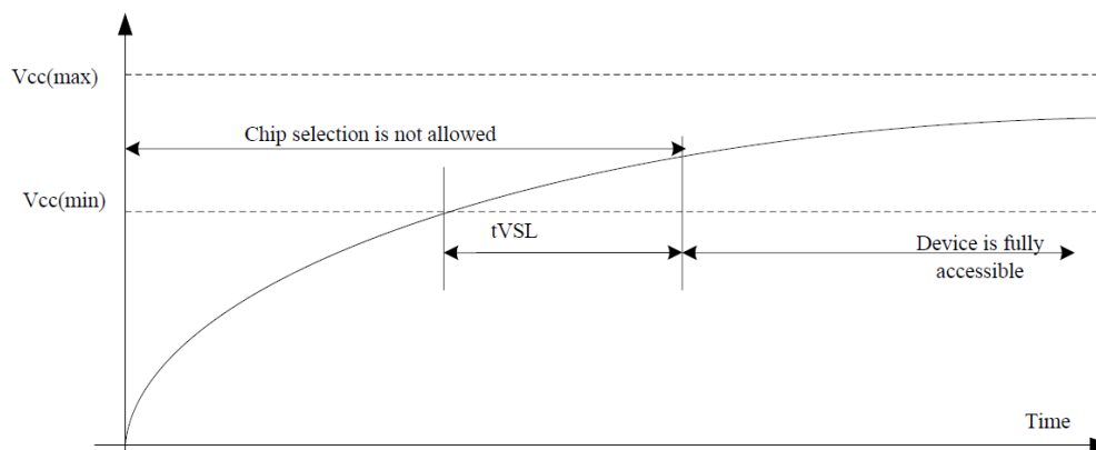
Figure40. Power-up Timing and Voltage Levels
