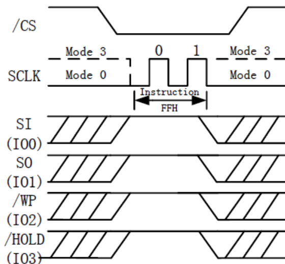
Figure39. Exit QPI Instruction (QPI Mode only)
