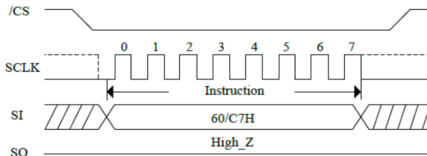
Figure36. Chip Erase Sequence Diagram
