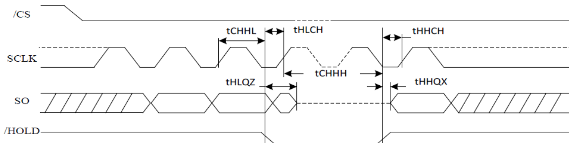
Figure 43. Output Timing
