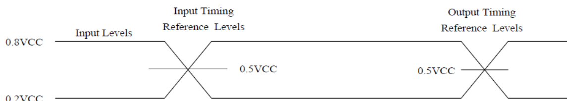
Figure41. AC Measurement I/O Waveform
