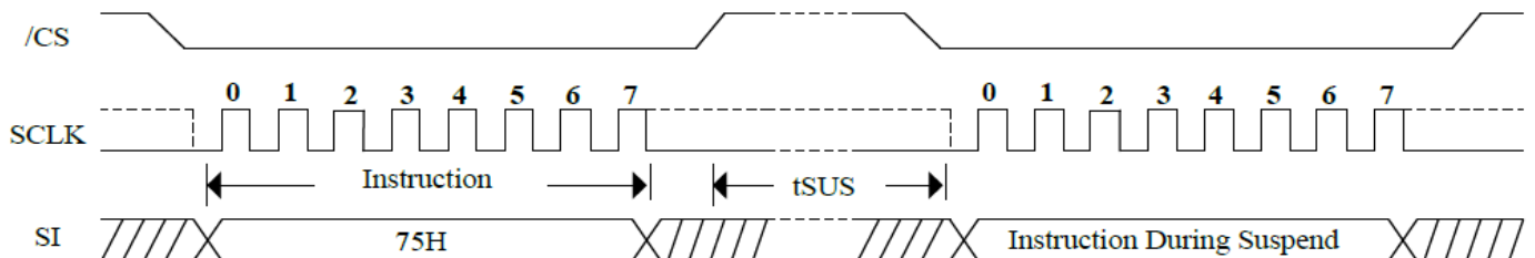
Figure37. Erase/Program Suspend Command Sequence
