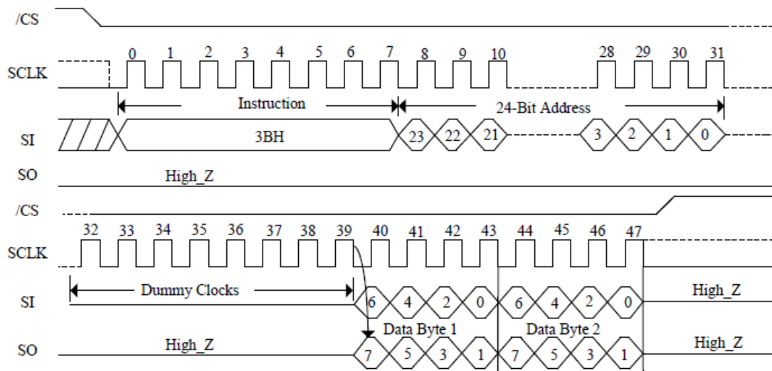
Figure9. Dual Output Fast Read Sequence Diagram
