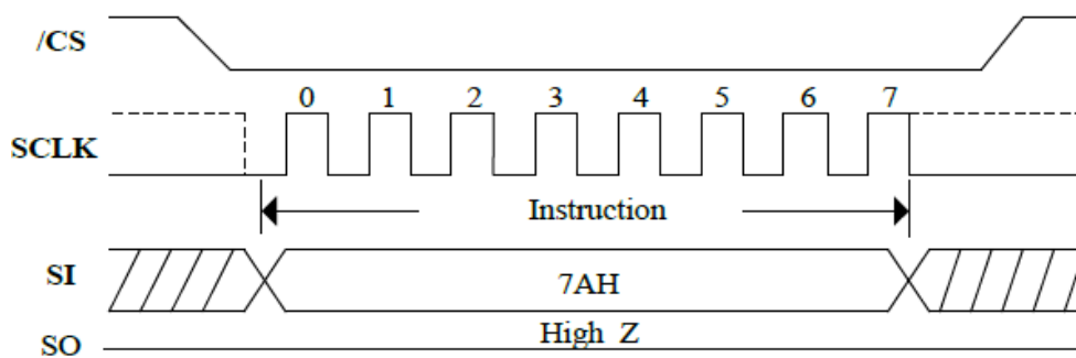
Figure38. Erase/Program Resume Command Sequence
