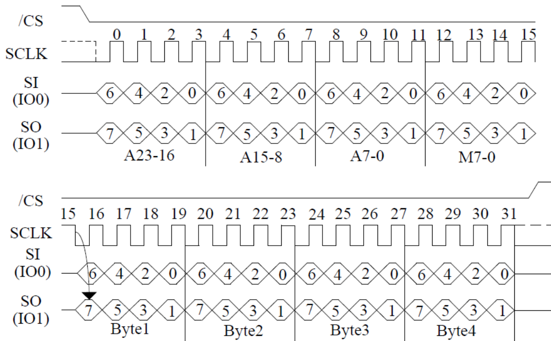
Figure12. Dual I/O Fast Read Sequence Diagram (Previous command set (M5-4) =(1,0))
