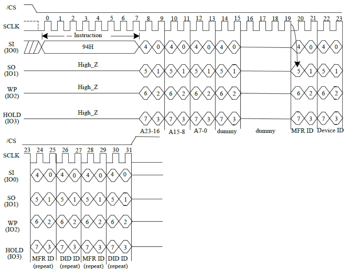
Figure20. Quad I/O Read Manufacture ID/ Device ID Sequence Diagram
