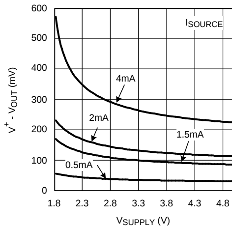
Figure 8. Output Positive Swing vs. V_{\text{SUPPLY}}
