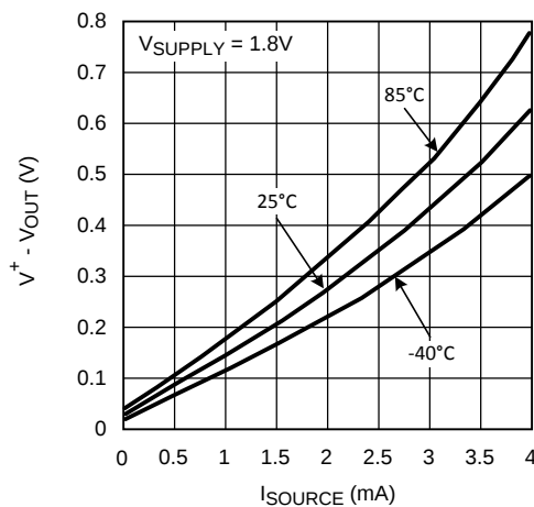
Figure 10. Output Positive Swing vs. I_{\text{SOURCE}}
