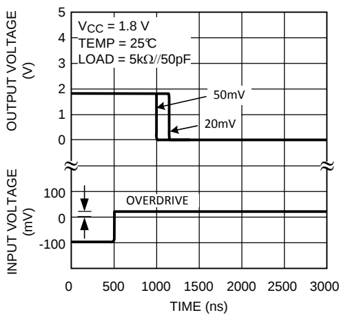
Figure 17. Propagation Delay ( t_{PHL} )
