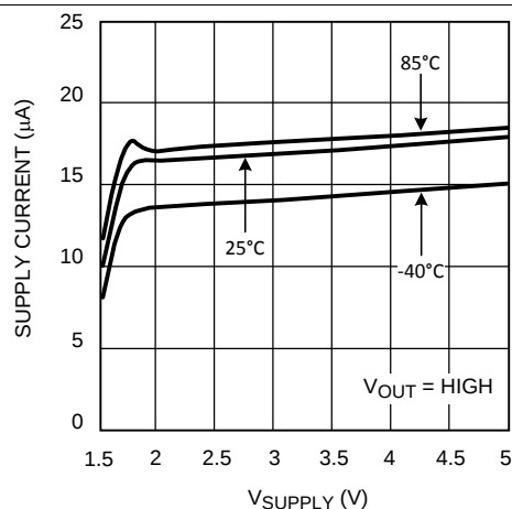
Figure 6. Supply Current vs. Supply Voltage (LMV7272)
