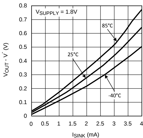
Figure 11. Output Negative Swing vs. I_{\text{SINK}}
