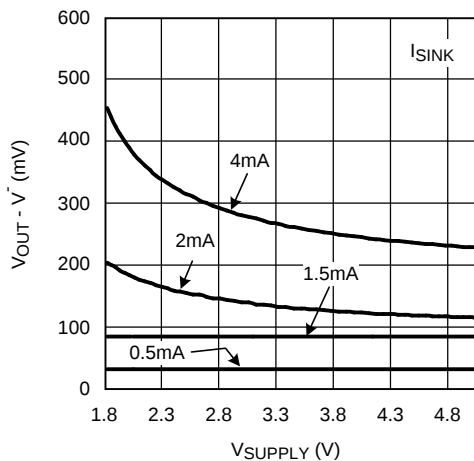
Figure 9. Output Negative Swing vs. V_{\text{SUPPLY}}
