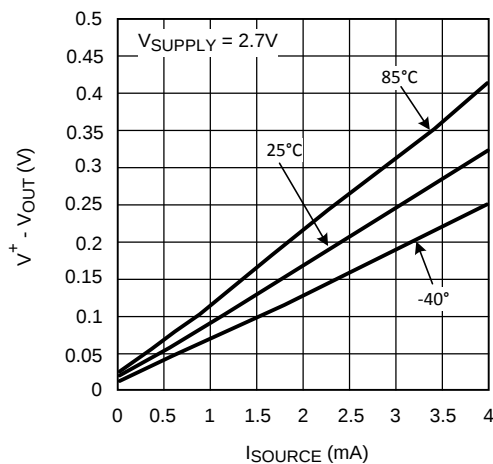
Figure 12. Output Positive Swing vs. I_{\text{SOURCE}}
