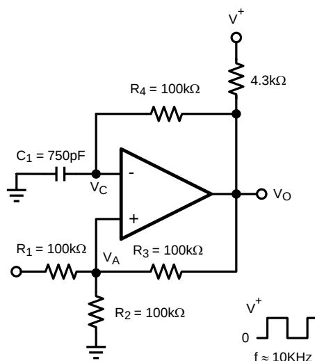
Figure 35. Square Wave Oscillator Application
