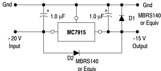
Figure 11. Protection Diodes
