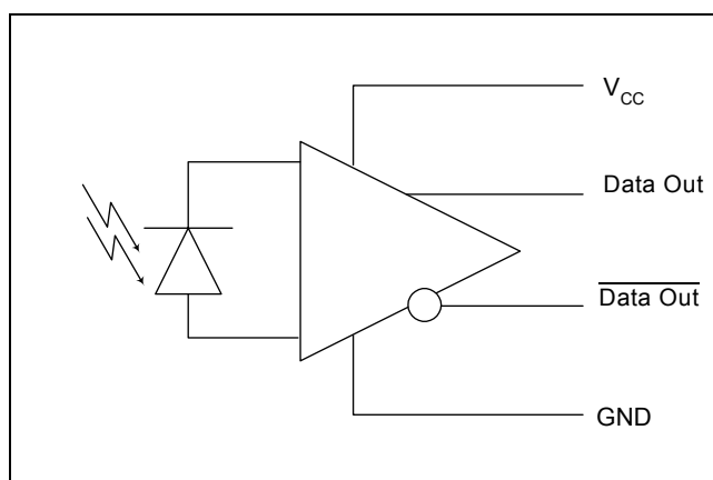
Figure 2 - Functional Schematic
