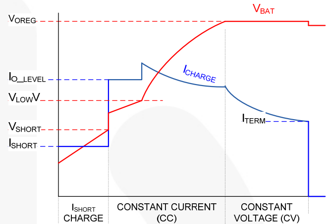
Figure 33. Charge Curve, I CHARGE Not Limited by I INLIM
