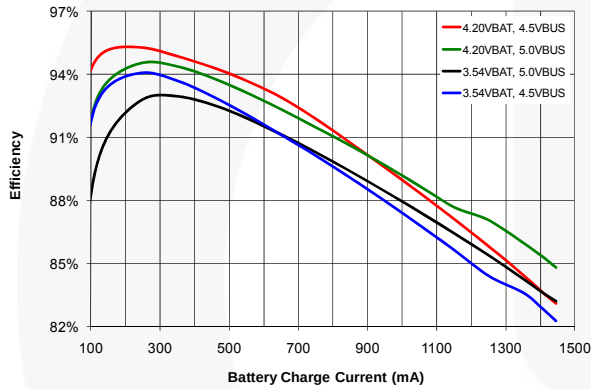
Figure 8. Charger Efficiency, No I_{INLIM} , I_{CHARGE}=1450\text{ mA}
