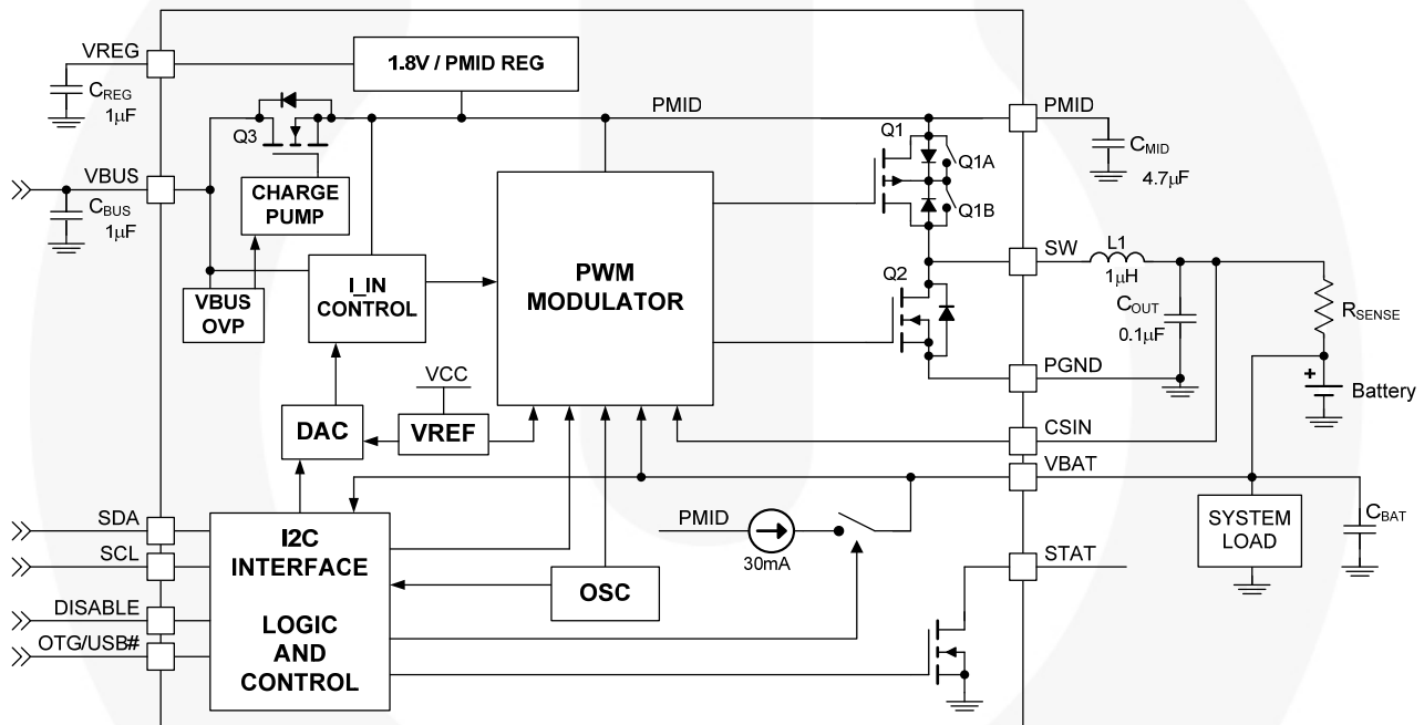
Figure 2. IC and System Block Diagram
