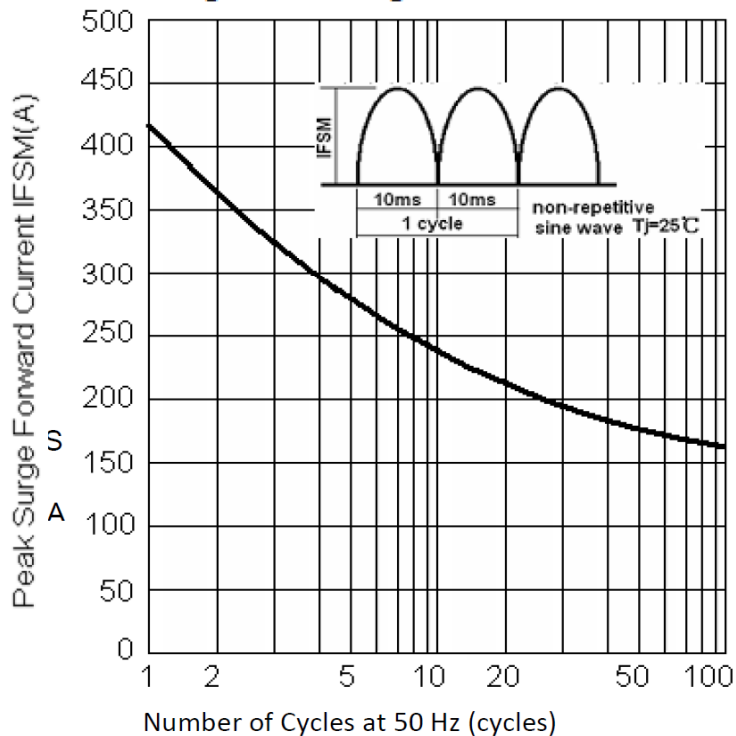
Fig.3: Max. Surge Current
