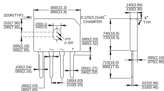
Dimensions in inches and (millimeters)
