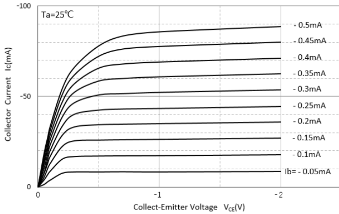
Static Characteristic
