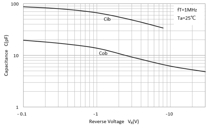
C_{ob}/C_{ib}-V_{CB}/V_{EB}
