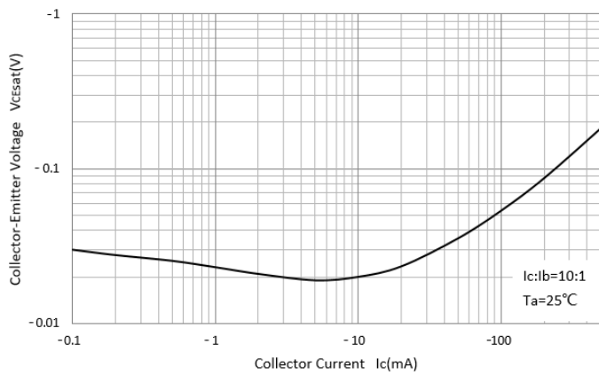
Collector-Emittor Saturation Voltage
