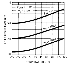
Output Swing
