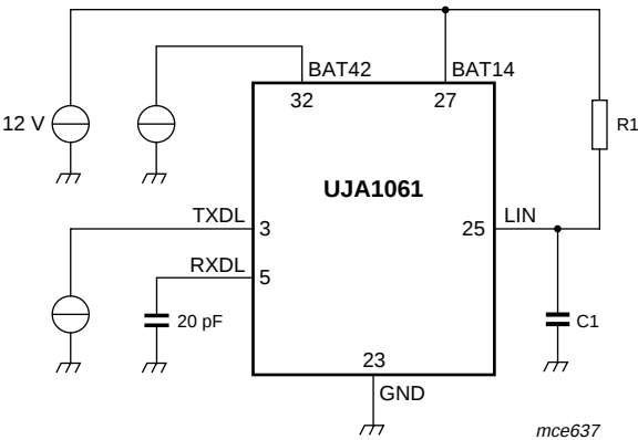
Fig.17 Timing test circuit for LIN-transceiver.
