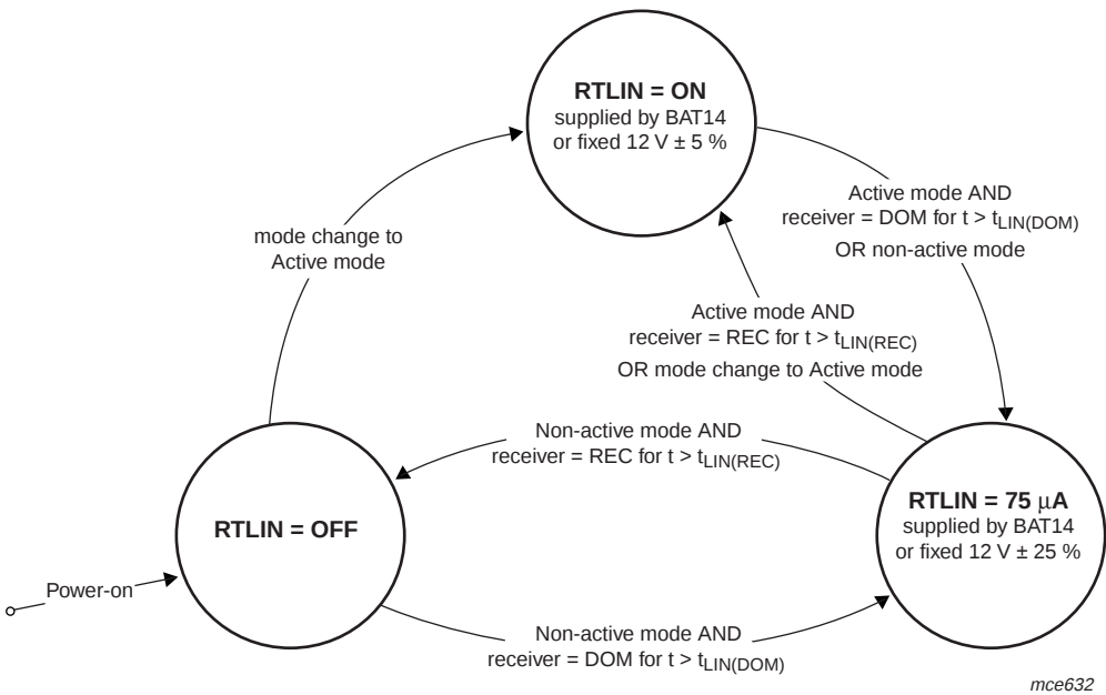
Fig.11 States of the RTLIN pin.
