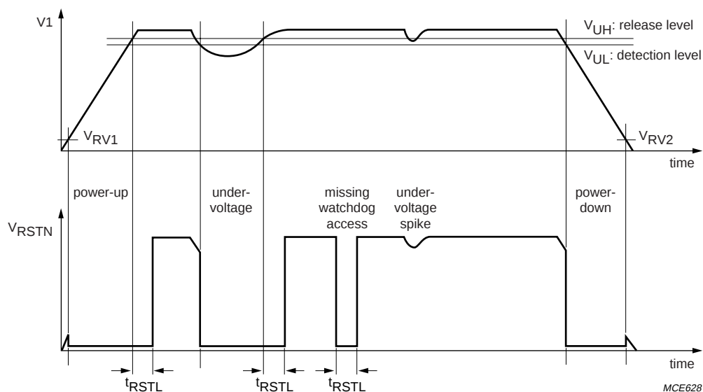
Fig.7 Reset pin behaviour.
