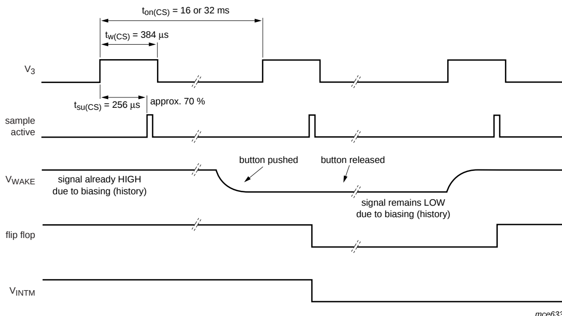
Fig.12 Pin WAKE, cyclic sampling via V3.
