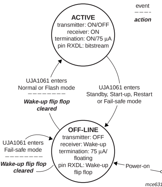
Fig.10 States LIN transceiver.
