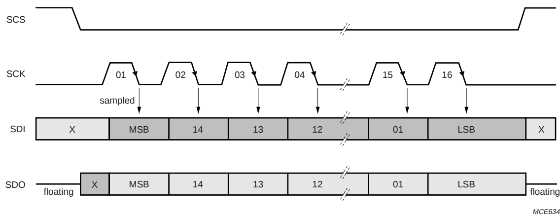
Fig.13 SPI timing protocol.
