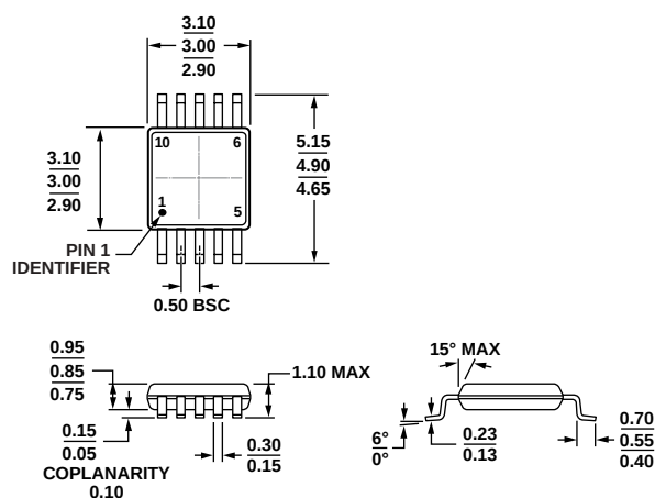
Figure 46. 10-Lead Mini Small Outline Package [MSOP] (RM-10) Dimensions shown in millimeters
