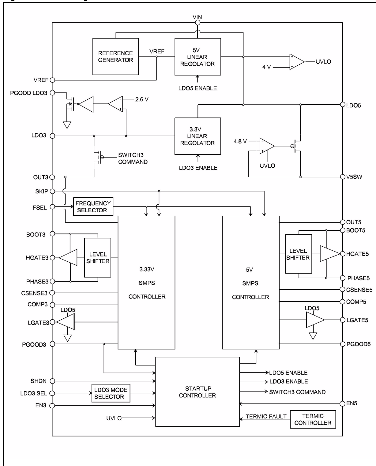
Figure 3. Block diagram
