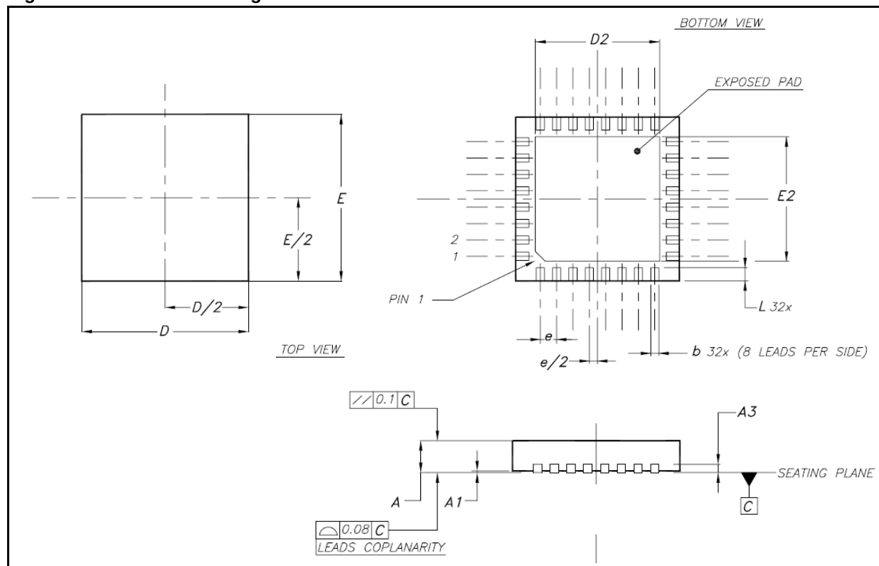
Figure 4. Scheme Drawings
