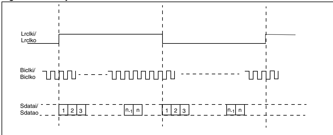
Figure 6. Left justified
