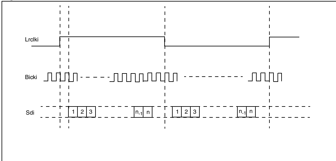
Figure 5. I 2 S
