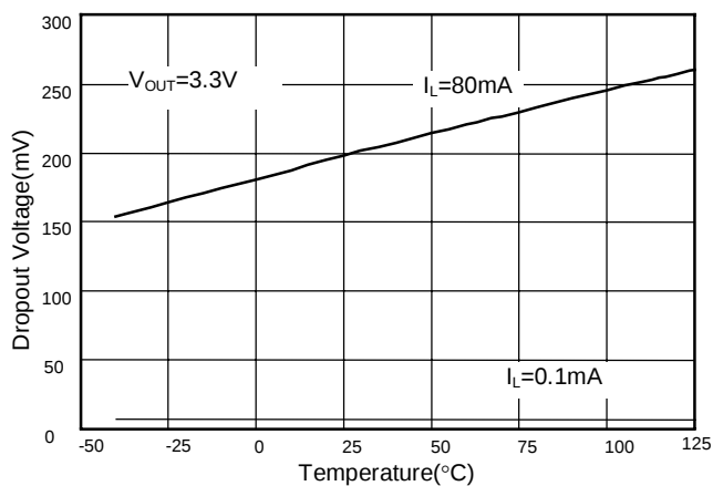
Dropout Voltage vs Temperature
